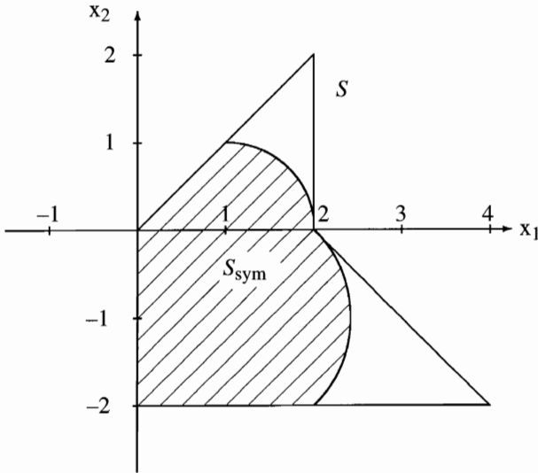
Fig. 3. The solution sets S and S_{\text{sym}} of Example 3
