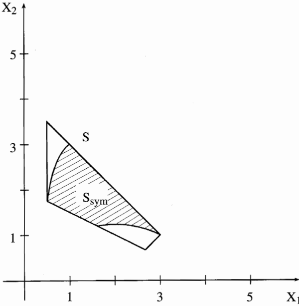
Fig. 2. The solution sets S and S_{\text{sym}} of Example 2
