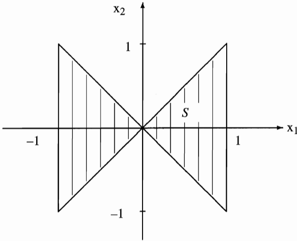
Fig. 1. The solution set S of Example 1
