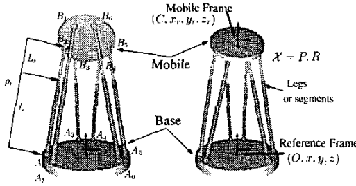
Fig. 1. Gough platform.
